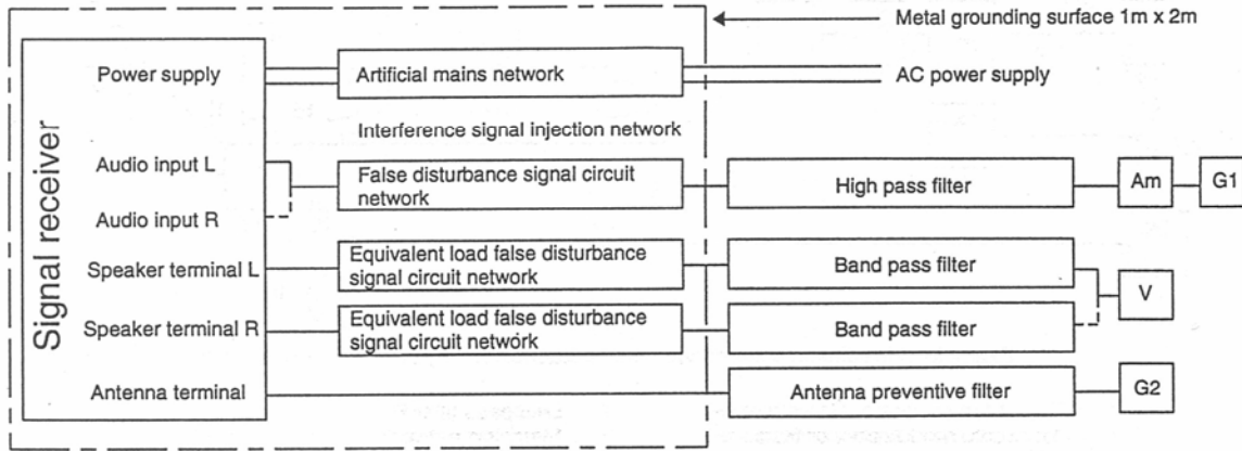
Example of immunity test measurement layout
